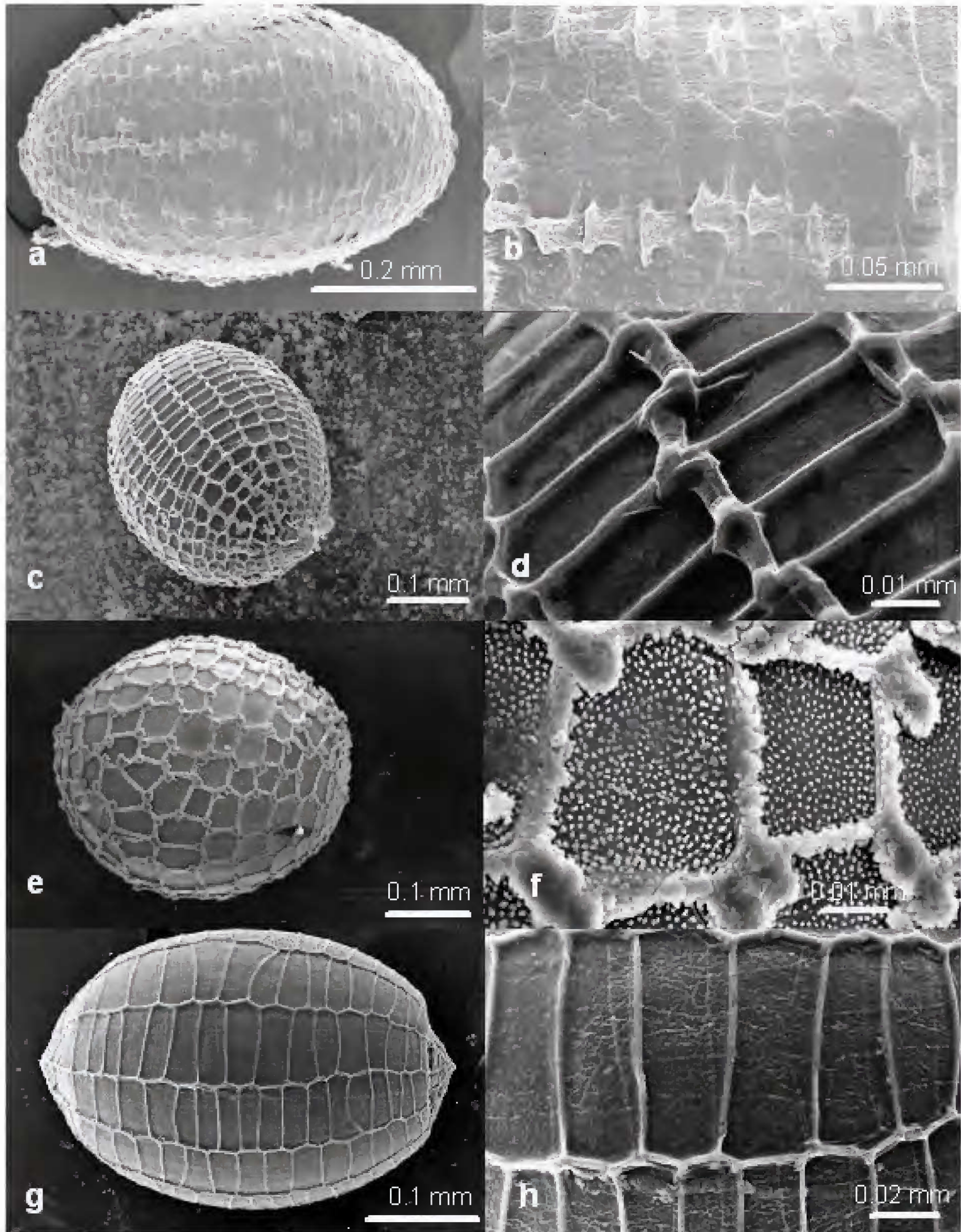
Fig. 9. Seed and seed surface: Eriocaulon setaceum a, b; E. spectabile c, d; E. tortuosum e, f; E. tricornum g, h. Material used: a-b from Wilson 339; c-d from Mueller MEL1501981; e-f from Dunlop 3725; g-h from Egan 2177.
